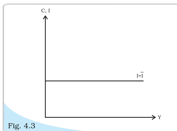
Investment function with I as autonomous.
